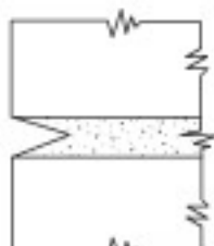
Fig. 9-5. Improperly prepared joint. — furrow should be eliminated.
